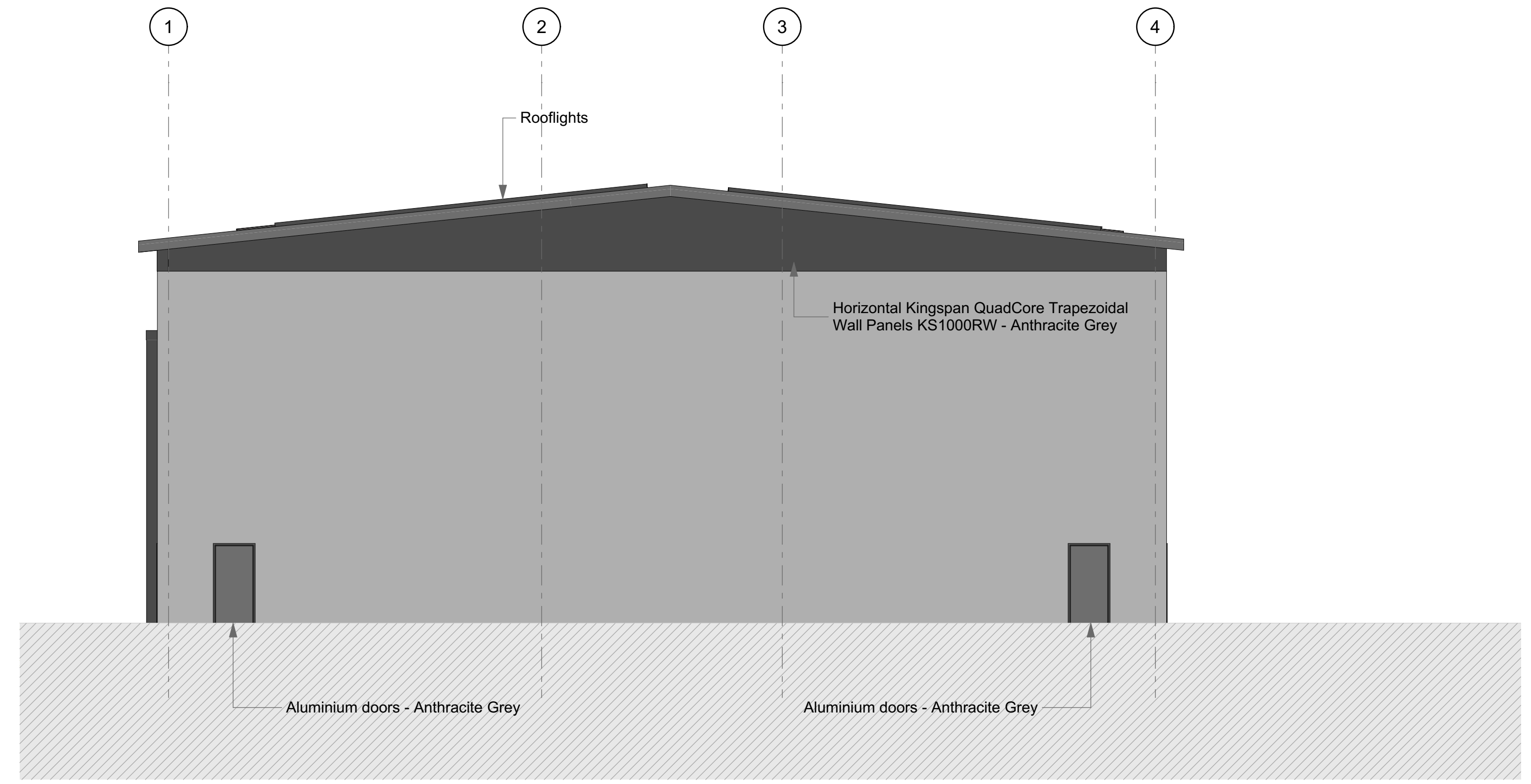
E-3.3 Elevation 1:100
