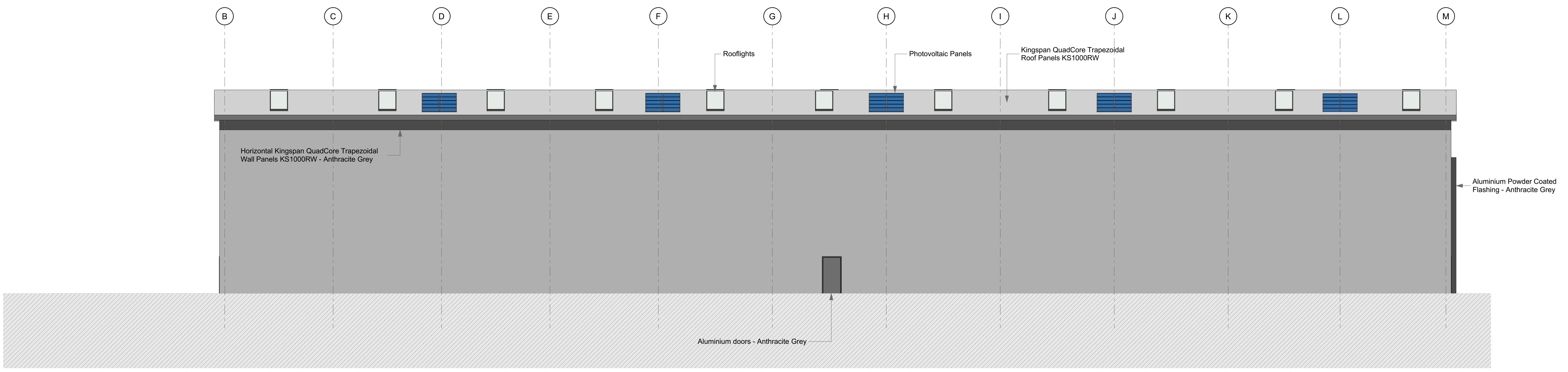
E-3.4 Elevation 1:100
