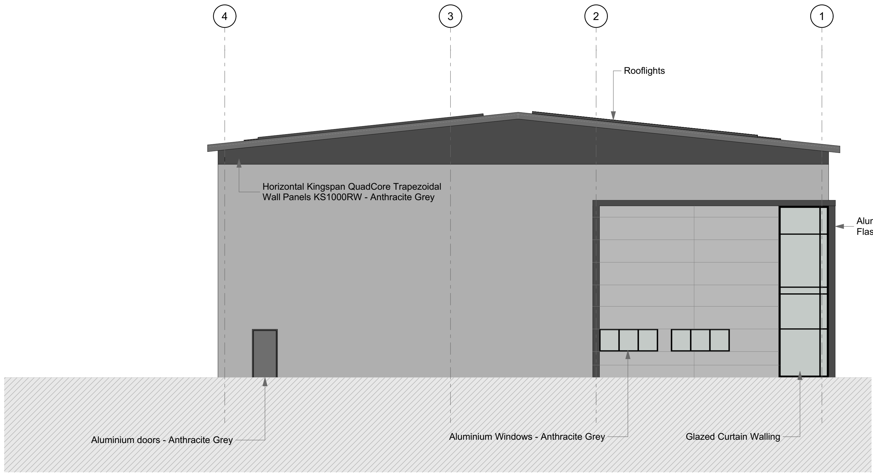
E-3.2 Elevation 1:100
